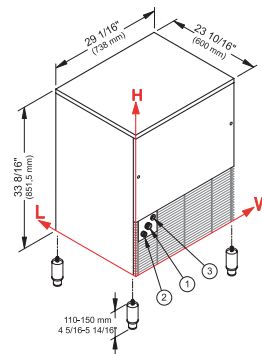
Adjustable feet 4 5/16" – 5 14/16"
