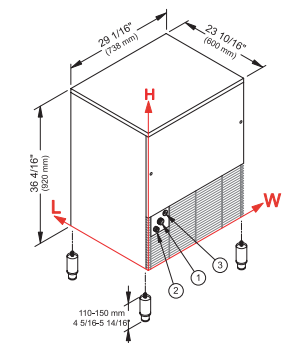
Adjustable feet 4 5/16" – 5 14/16"
