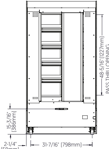
BACK VIEW WITH SWING DOOR
