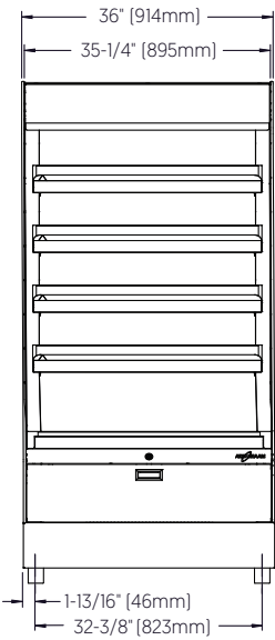
FRONT WITH FEET
